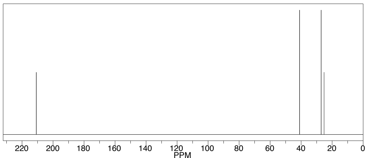
C-13 NMR of cyclohexanone
