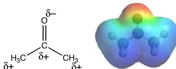
Two representations of acetone showing the distribution of charge
