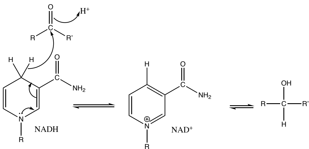
Reduction of a carbonyl by NADH by delivery of \text{H}^- to the carbonyl carbon
