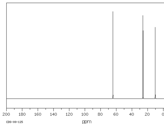
C-13 Spectrum of 1-propanol
