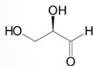
D-Glyceraldehyde
