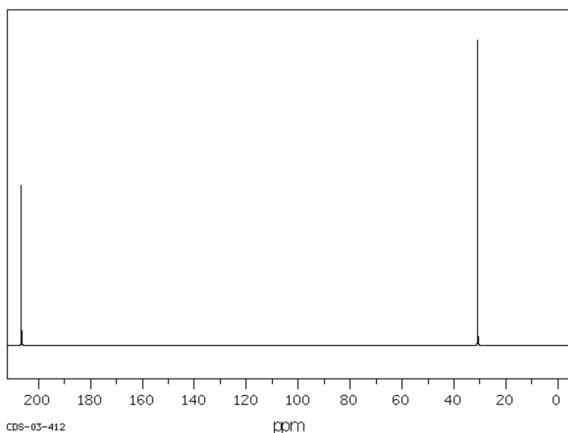
C-13 NMR spectrum of acetone
