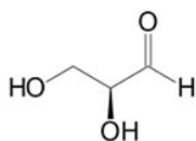
L-Glyceraldehyde
