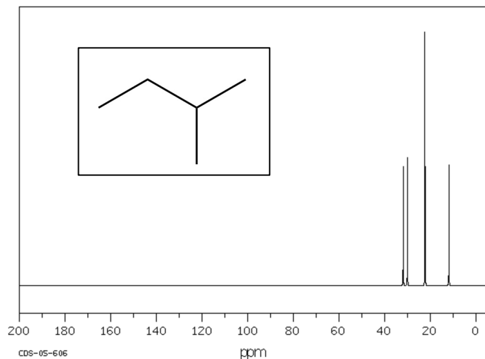
C-13 NMR of 2-methylbutane
