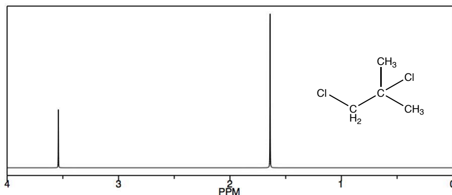
H-1 NMR Spectrum of 1,2-dichloro-2-methylpropane
