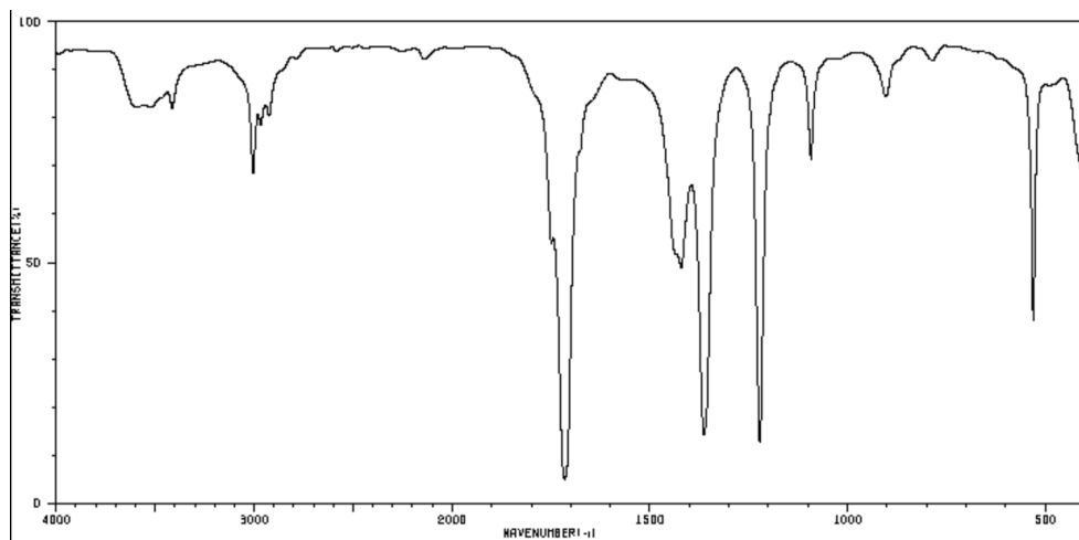
InfraRed Spectrum of Acetone ( \text{CH}_3\text{COCH}_3 )
