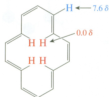
[14]Annulene
